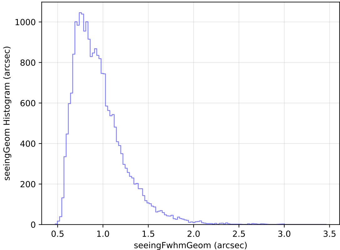
internal_u_expt45_nscale1.1v3.4_10yrs Yr 1 g band: seeingGeom Histogram
