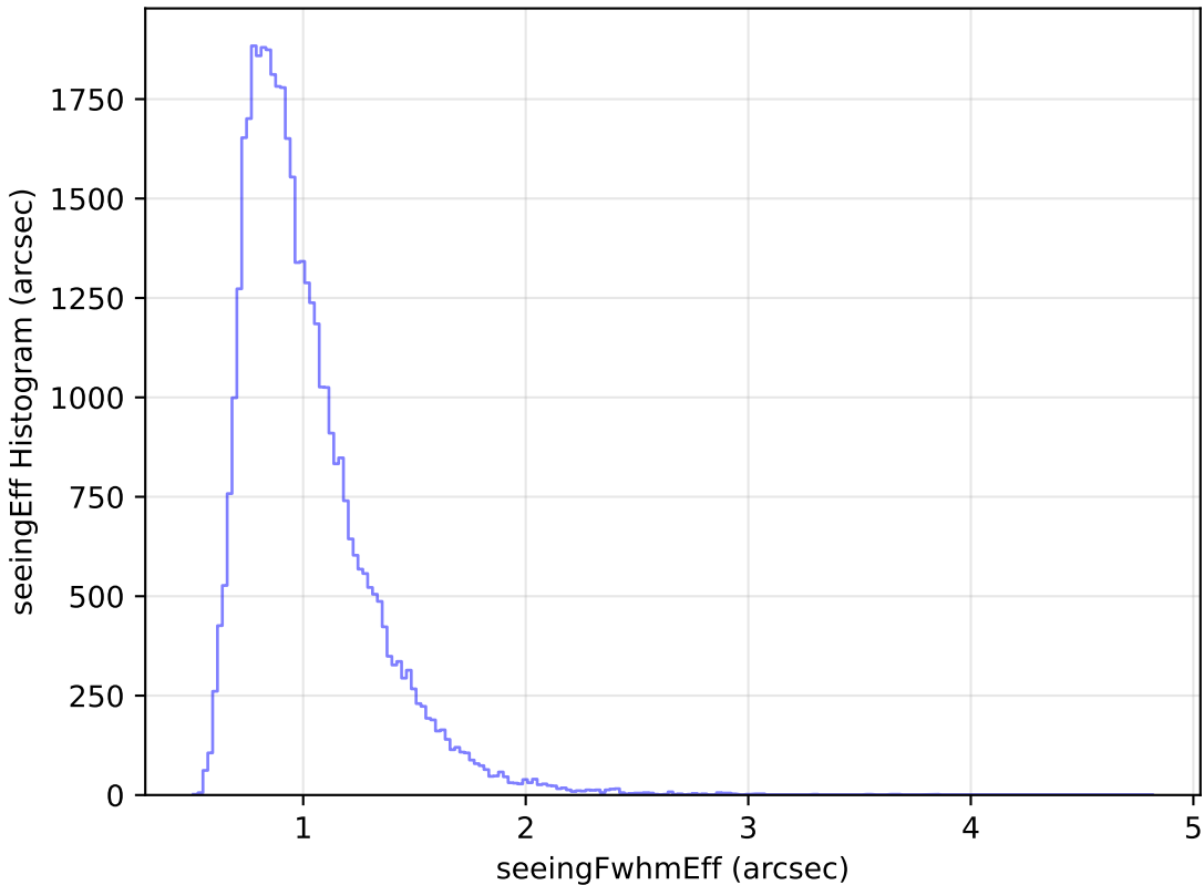
internal_u_expt45_nscale1.1v3.4_10yrs Yr 1 z band: seeingEff Histogram
