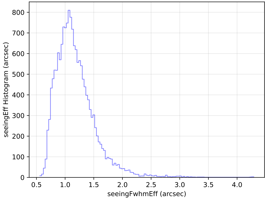
internal_u_expt45_nscale1.1v3.4_10yrs Yr 1 u band: seeingEff Histogram
