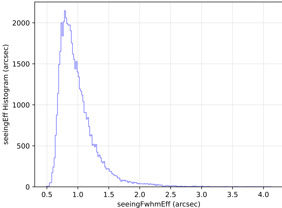
internal_u_expt45_nscale1.1v3.4_10yrs Yr 1 i band: seeingEff Histogram
