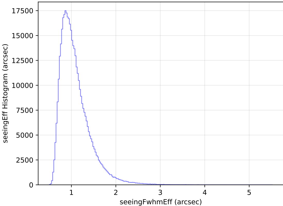
internal_u_expt45_nscale1.1v3.4_10yrs WFD z band: seeingEff Histogram
