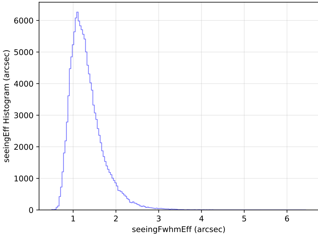
internal_u_expt45_nscale1.1v3.4_10yrs WFD u band: seeingEff Histogram
