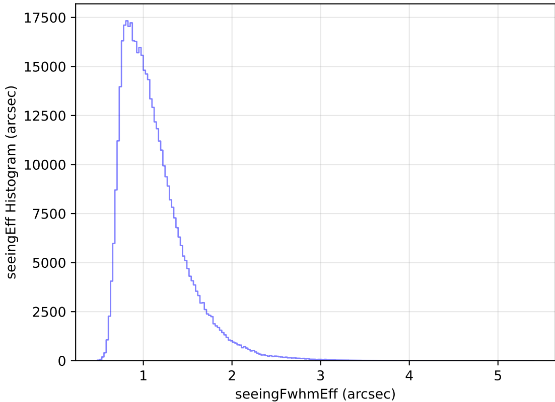
internal_u_expt45_nscale1.1v3.4_10yrs WFD r band: seeingEff Histogram
