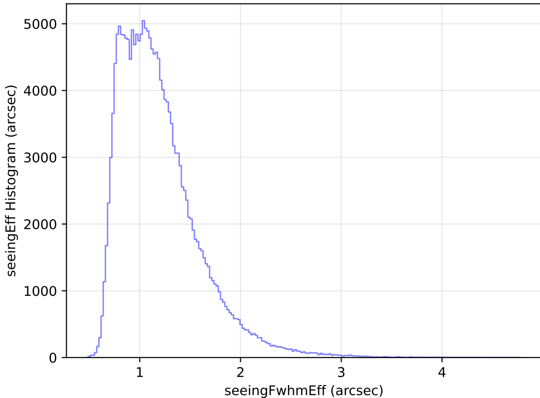
internal_u_expt45_nscale1.1v3.4_10yrs WFD g band: seeingEff Histogram
