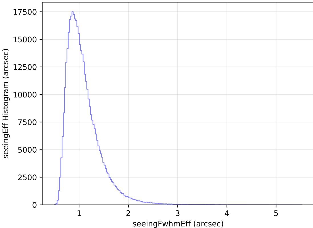
internal_u_expt45_nscale1.1v3.4_10yrs All sky z band: seeingEff Histogram
