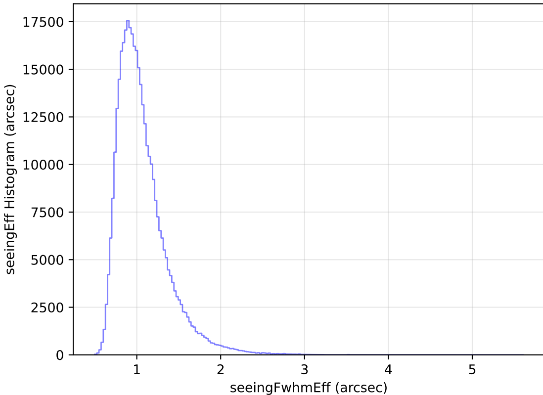
internal_u_expt45_nscale1.1v3.4_10yrs All sky y band: seeingEff Histogram
