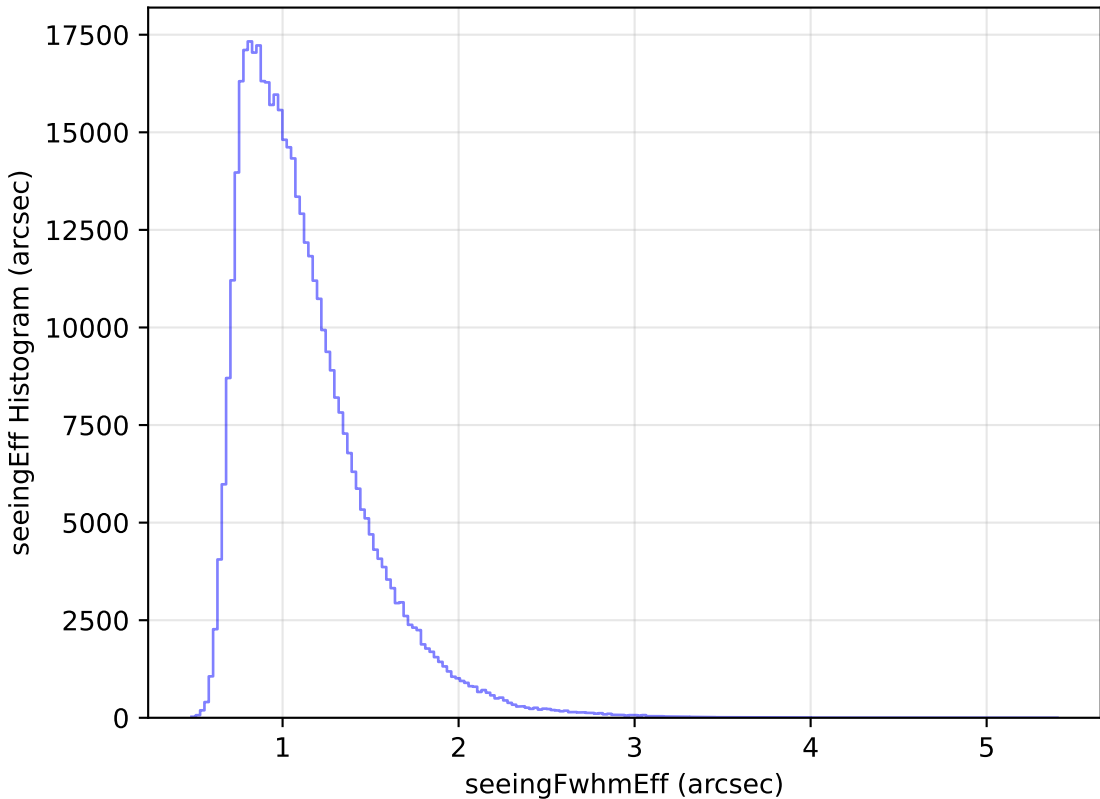
internal_u_expt45_nscale1.1v3.4_10yrs All sky r band: seeingEff Histogram
