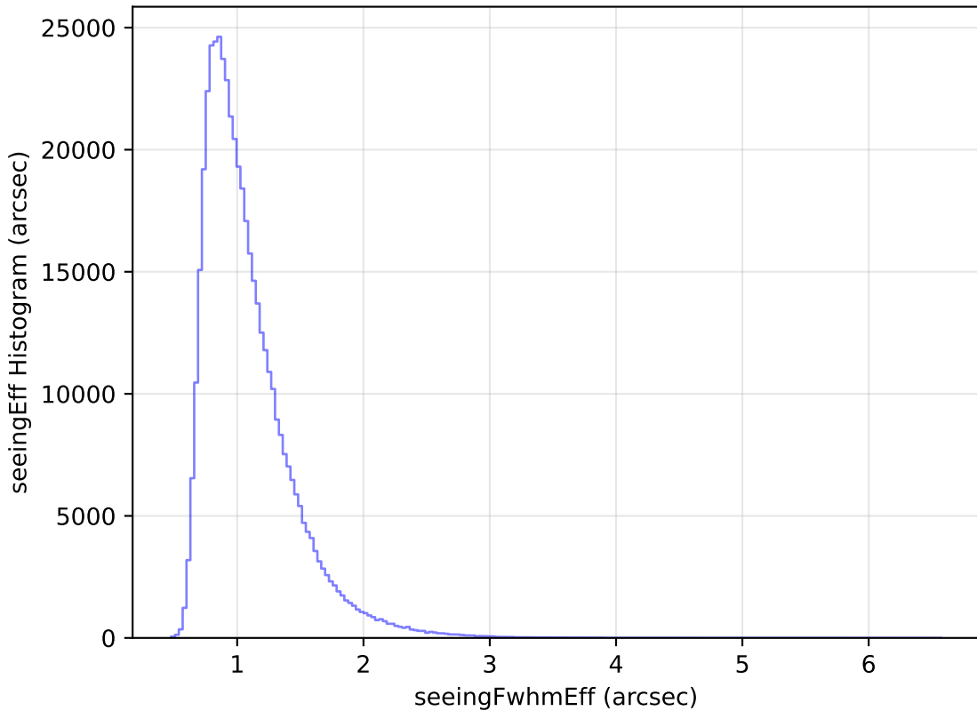
internal_u_expt45_nscale1.1v3.4_10yrs All sky i band: seeingEff Histogram
