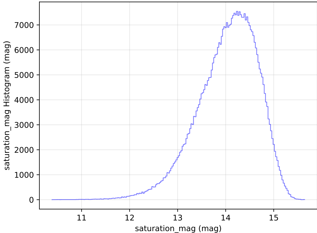
internal_u_expt45_nscale1.1v3.4_10yrs WFD z band: saturation_mag Histogram
