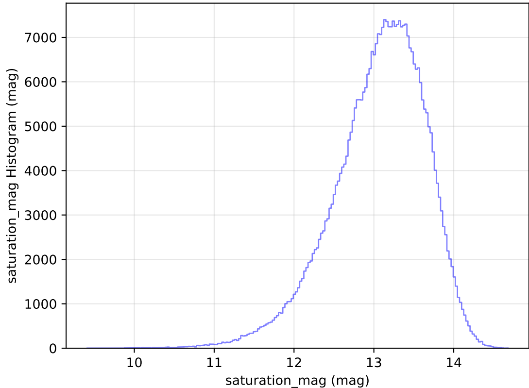
internal_u_expt45_nscale1.1v3.4_10yrs WFD y band: saturation_mag Histogram
