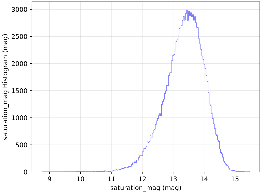
internal_u_expt45_nscale1.1v3.4_10yrs WFD u band: saturation_mag Histogram
