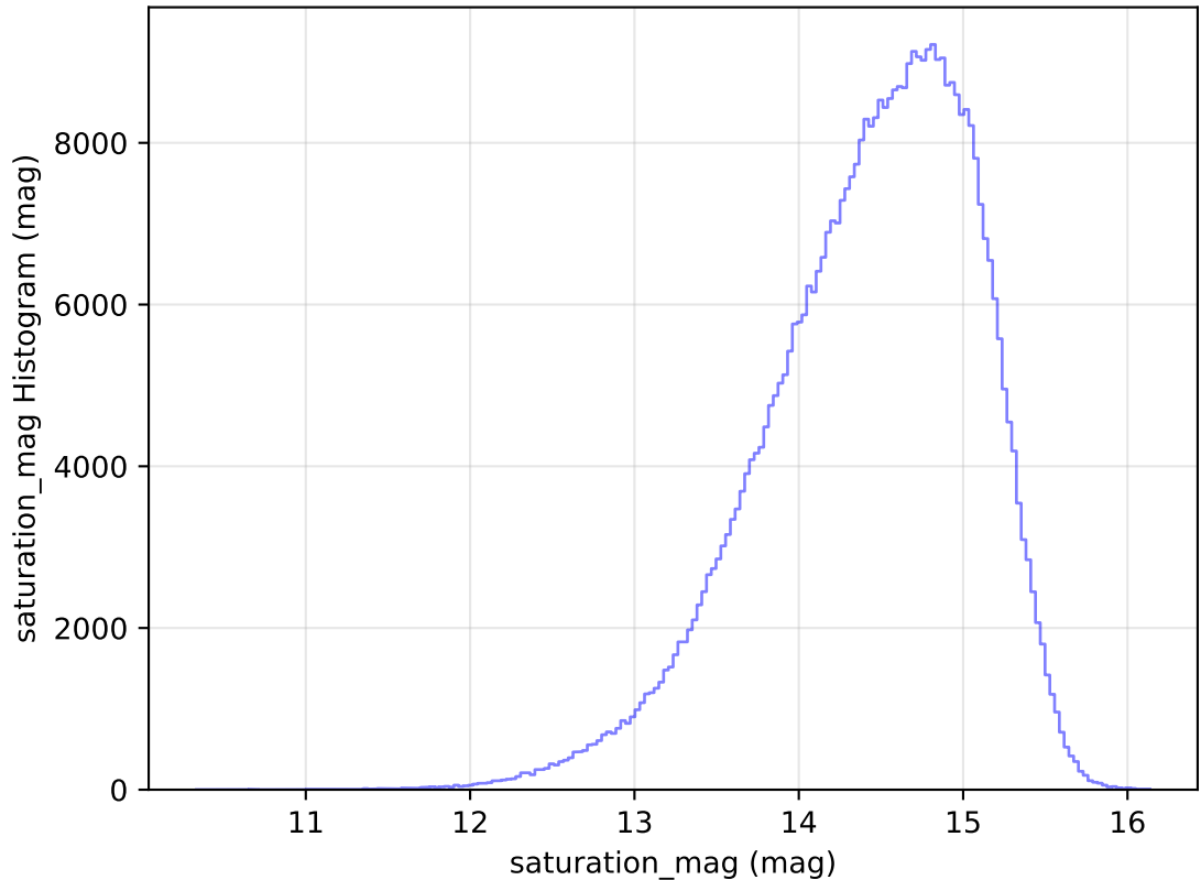
internal_u_expt45_nscale1.1v3.4_10yrs WFD i band: saturation_mag Histogram
