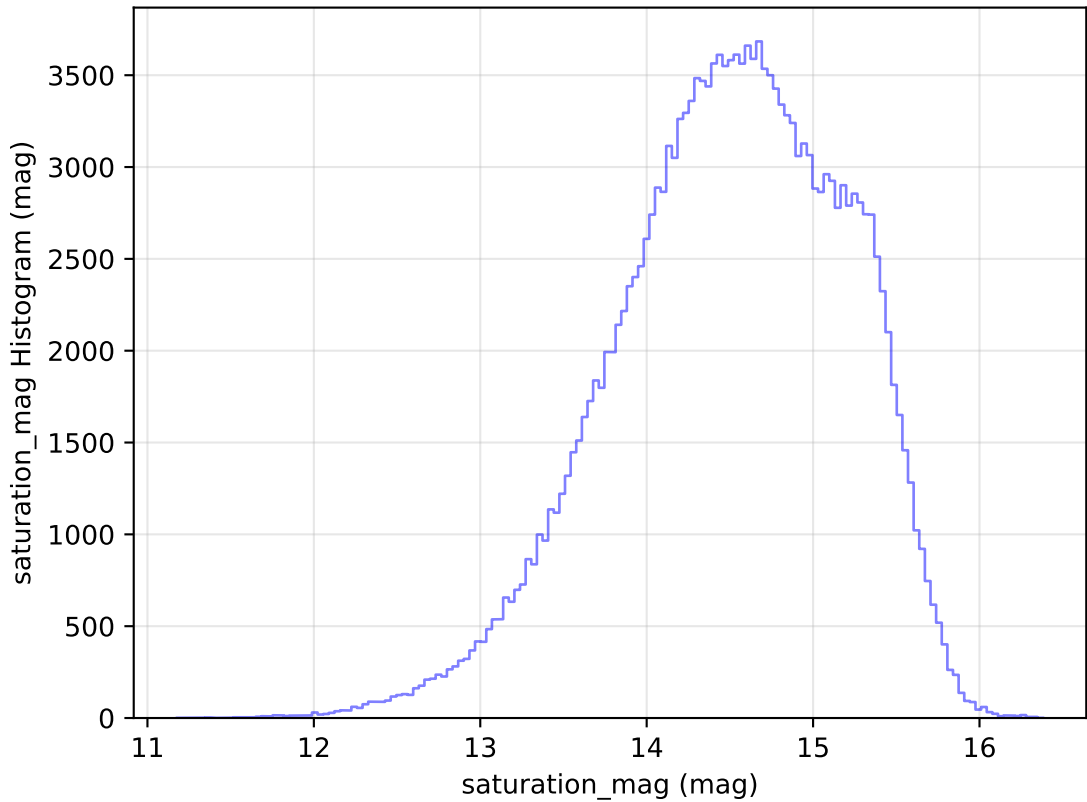
internal_u_expt45_nscale1.1v3.4_10yrs WFD g band: saturation_mag Histogram
