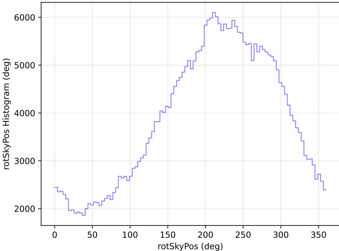
internal_u_expt45_nscale1.1v3.4_10yrs WFD y band: rotSkyPos Histogram
