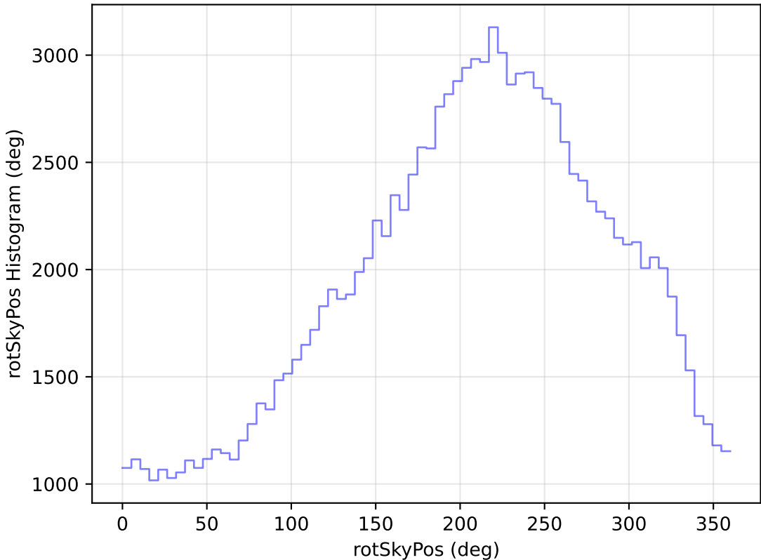
internal_u_expt45_nscale1.1v3.4_10yrs WFD u band: rotSkyPos Histogram
