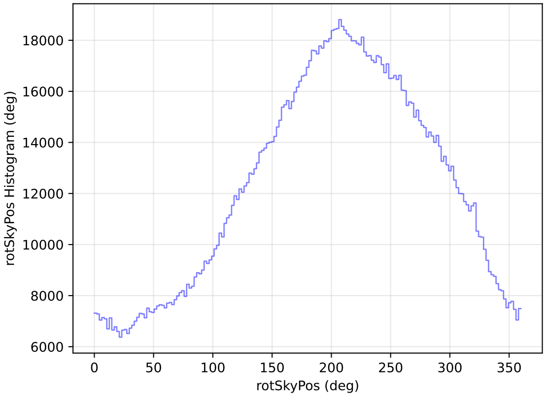
internal_u_expt45_nscale1.1v3.4_10yrs WFD all bands: rotSkyPos Histogram
