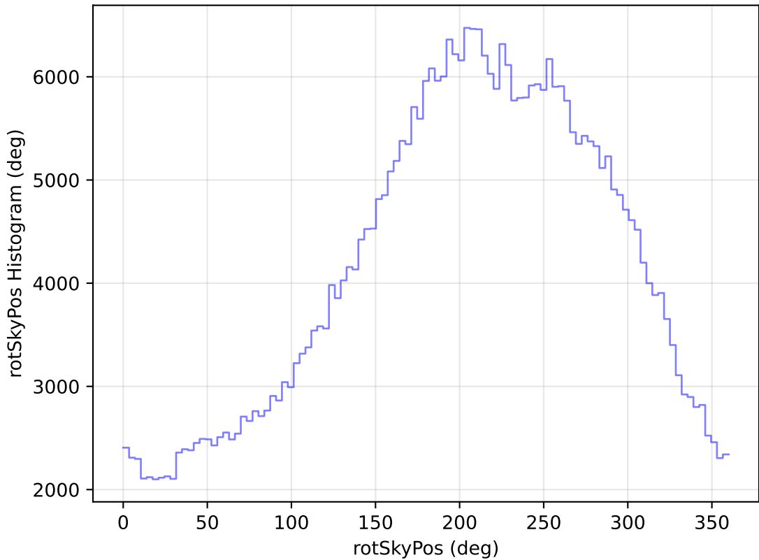
internal_u_expt45_nscale1.1v3.4_10yrs All sky z band: rotSkyPos Histogram
