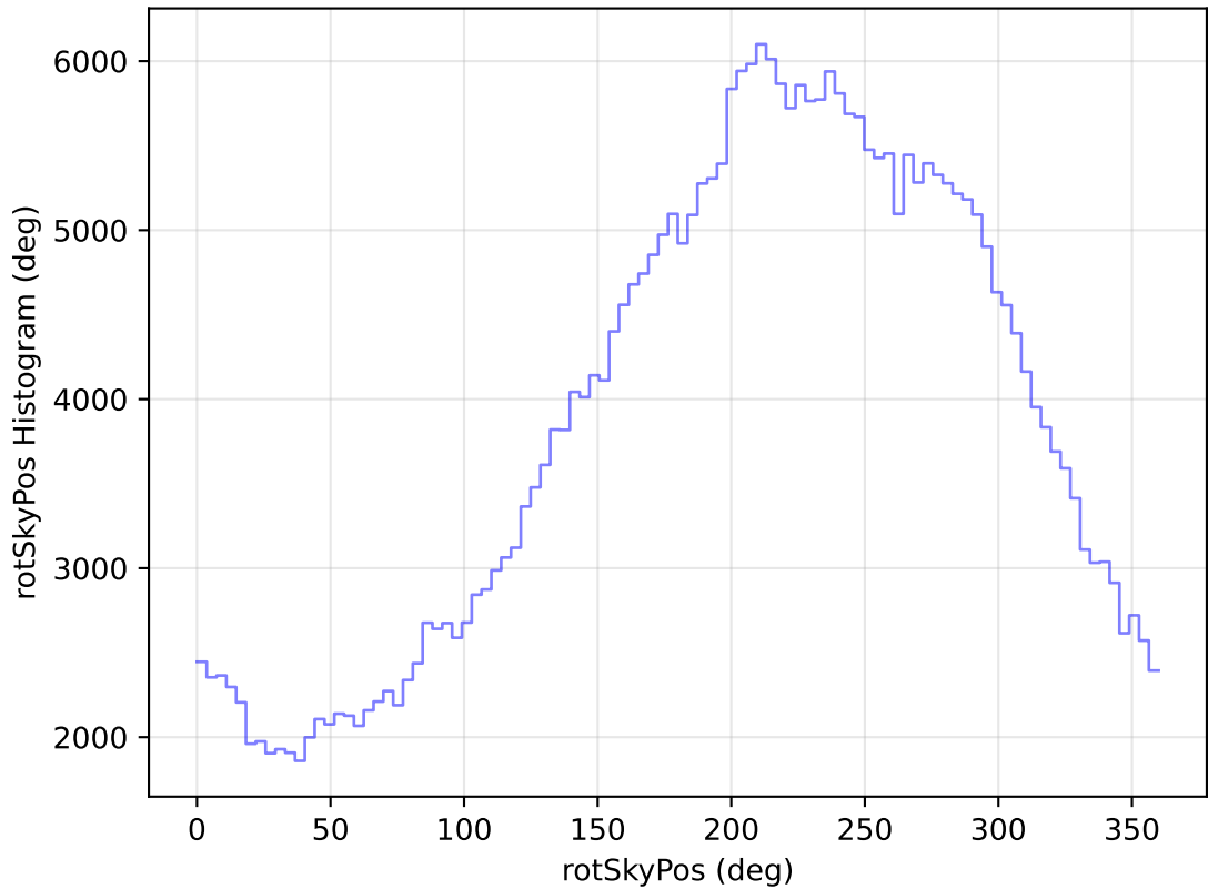
internal_u_expt45_nscale1.1v3.4_10yrs All sky y band: rotSkyPos Histogram
