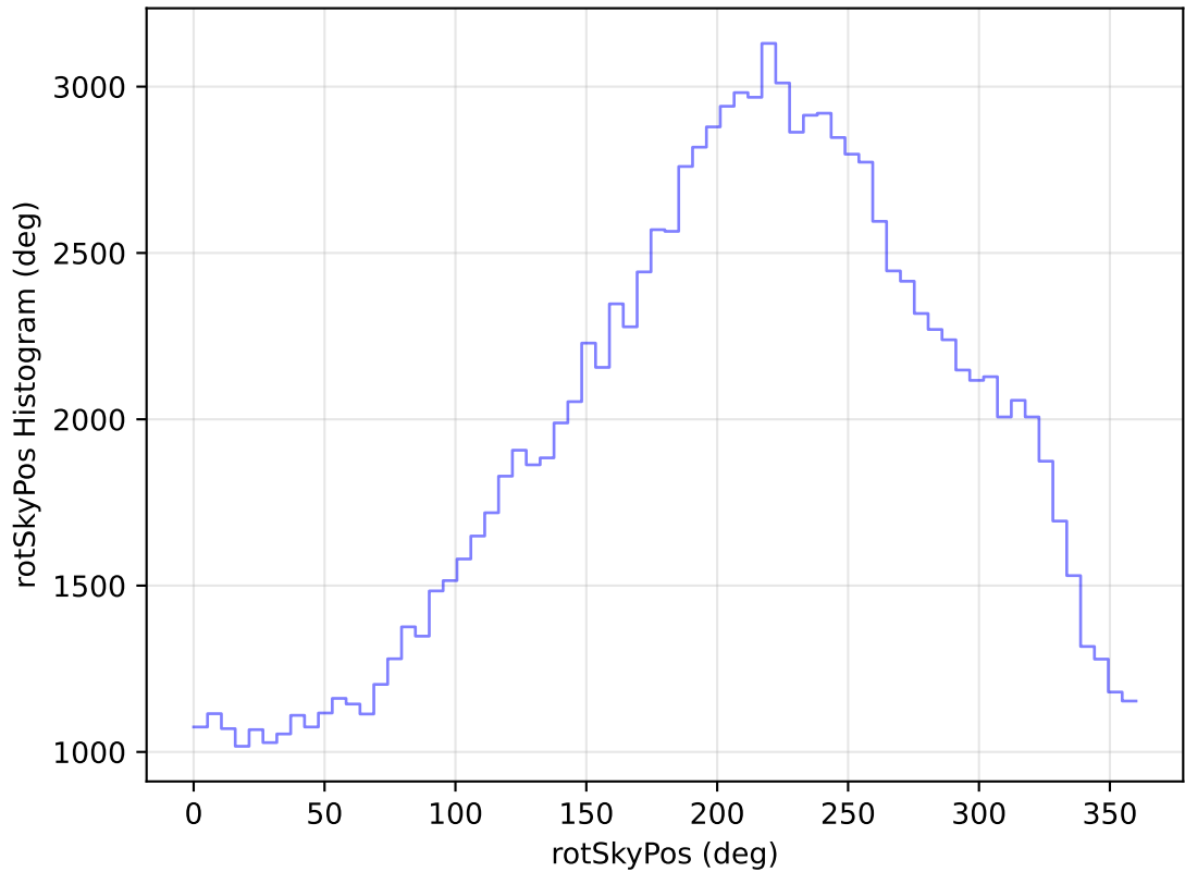
internal_u_expt45_nscale1.1v3.4_10yrs All sky u band: rotSkyPos Histogram
