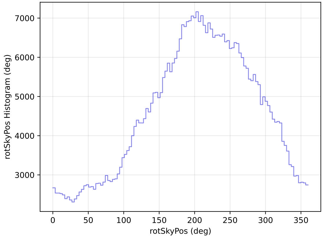
internal_u_expt45_nscale1.1v3.4_10yrs All sky i band: rotSkyPos Histogram
