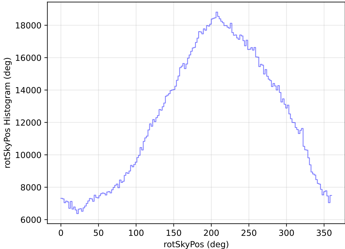
internal_u_expt45_nscale1.1v3.4_10yrs All sky all bands: rotSkyPos Histogram
