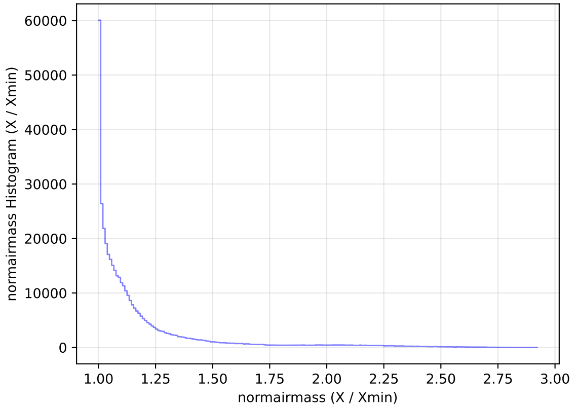
internal_u_expt45_nscale1.1v3.4_10yrs WFD z band: normairmass Histogram
