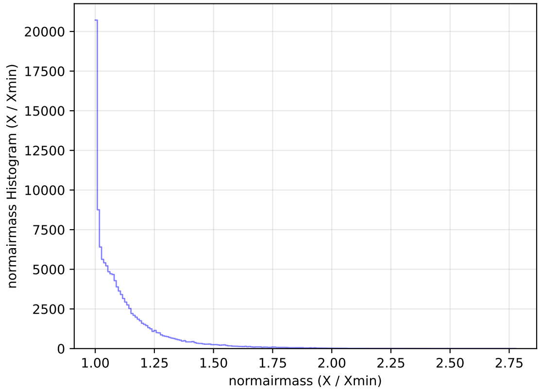
internal_u_expt45_nscale1.1v3.4_10yrs WFD u band: normairmass Histogram
