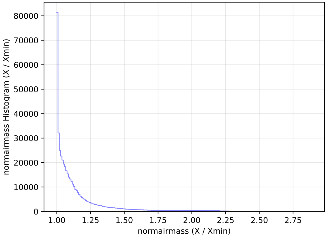
internal_u_expt45_nscale1.1v3.4_10yrs WFD r band: normairmass Histogram
