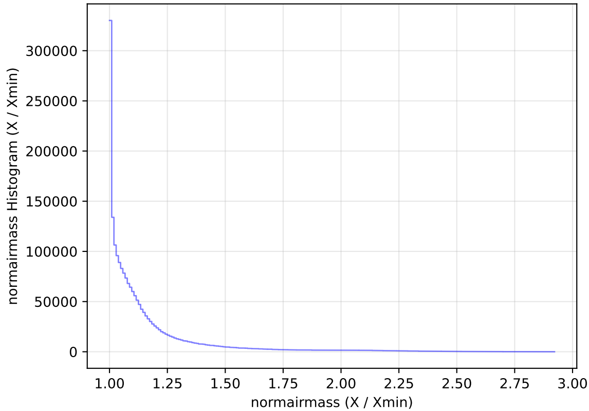
internal_u_expt45_nscale1.1v3.4_10yrs WFD all bands: normairmass Histogram
