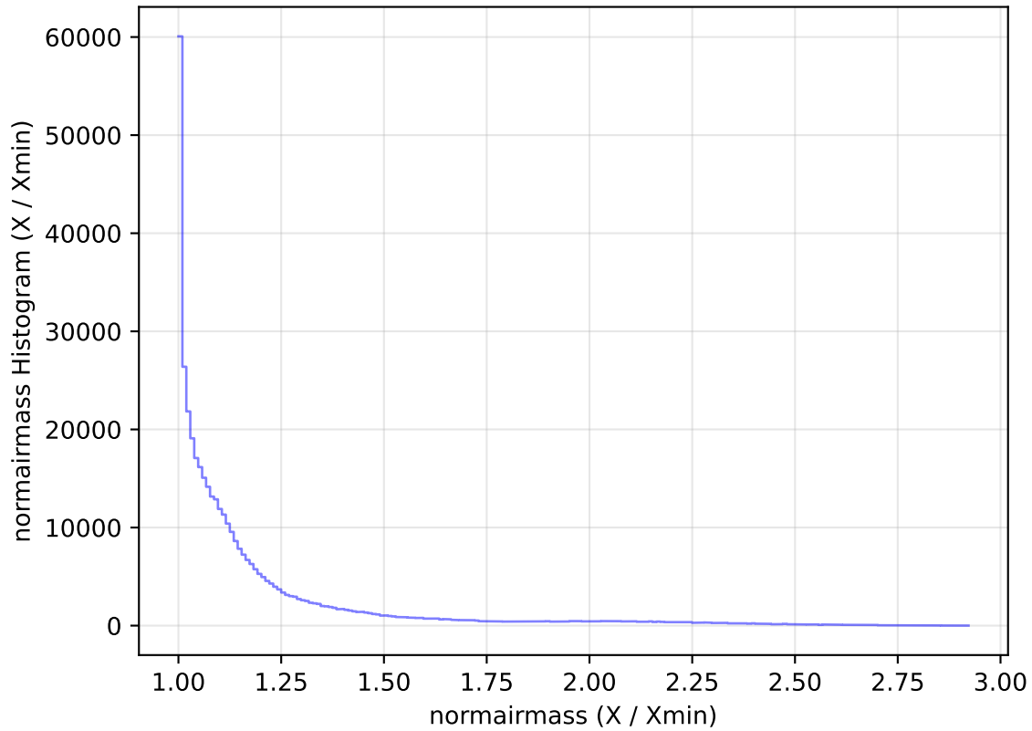
internal_u_expt45_nscale1.1v3.4_10yrs All sky z band: normairmass Histogram
