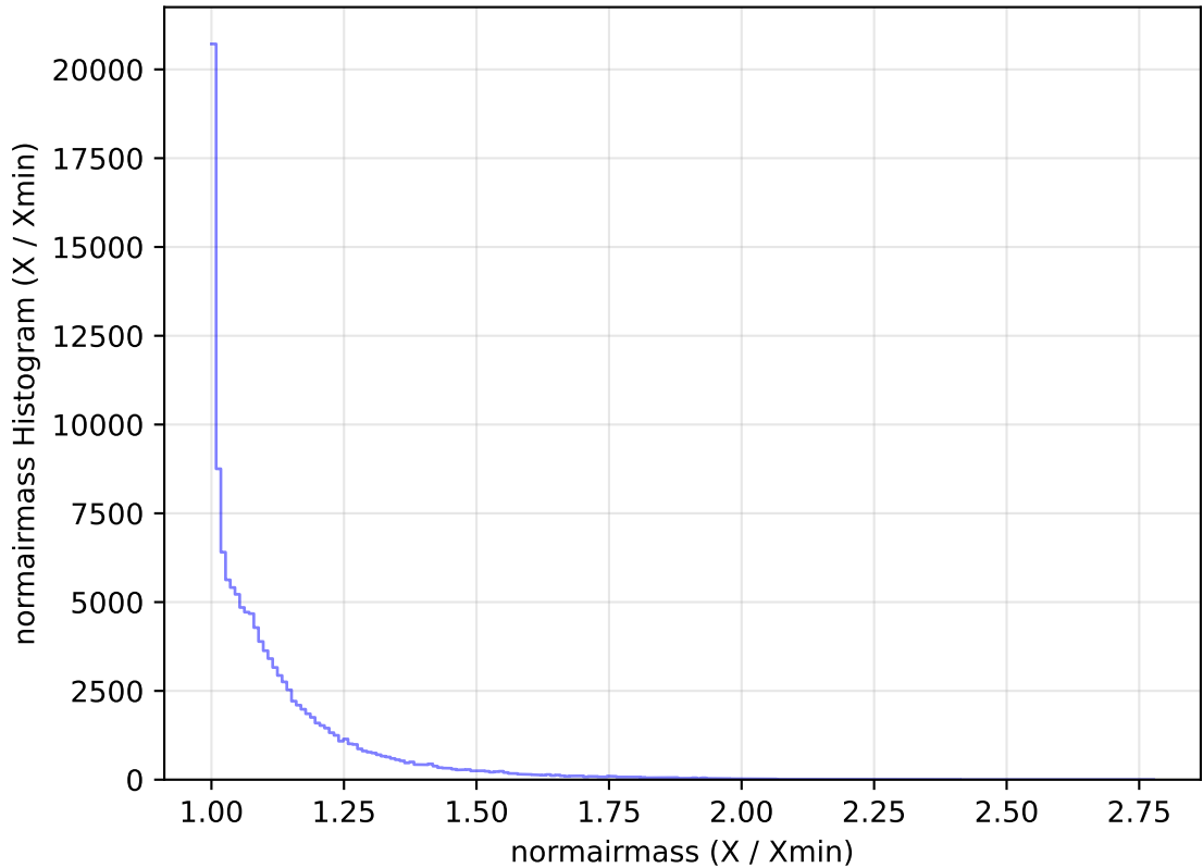
internal_u_expt45_nscale1.1v3.4_10yrs All sky u band: normairmass Histogram
