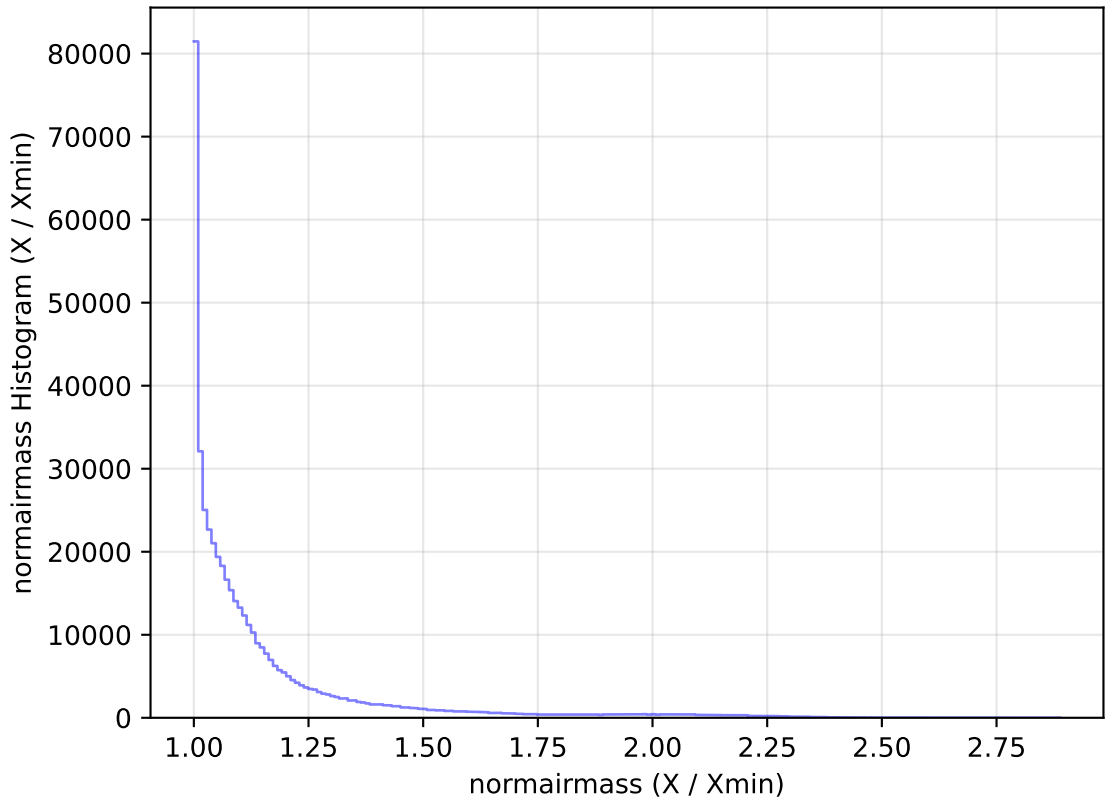
internal_u_expt45_nscale1.1v3.4_10yrs All sky r band: normairmass Histogram
