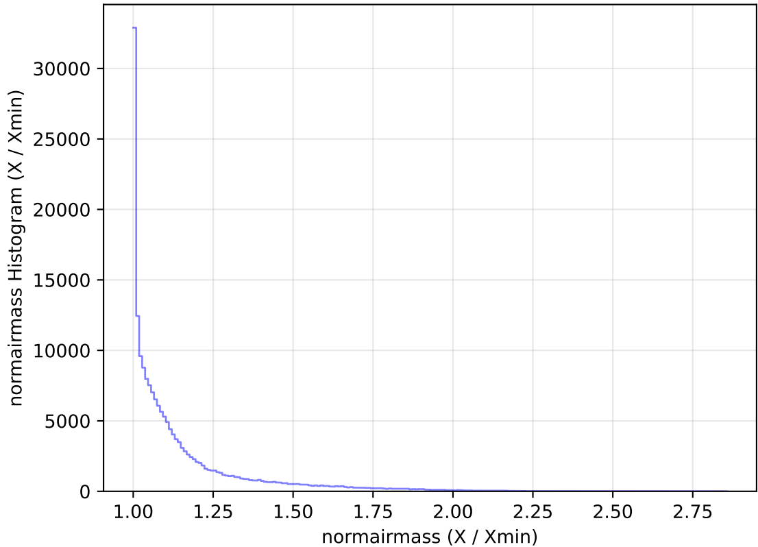
internal_u_expt45_nscale1.1v3.4_10yrs All sky g band: normairmass Histogram
