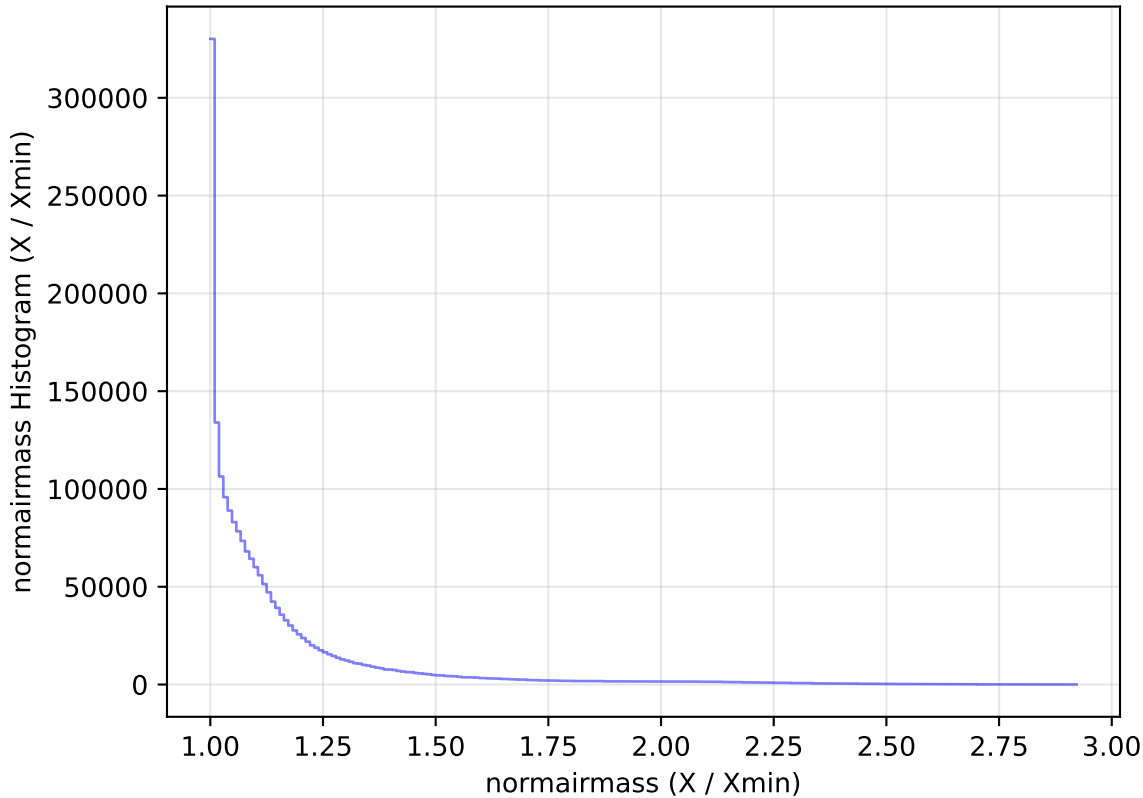
internal_u_expt45_nscale1.1v3.4_10yrs All sky all bands: normairmass Histogram
