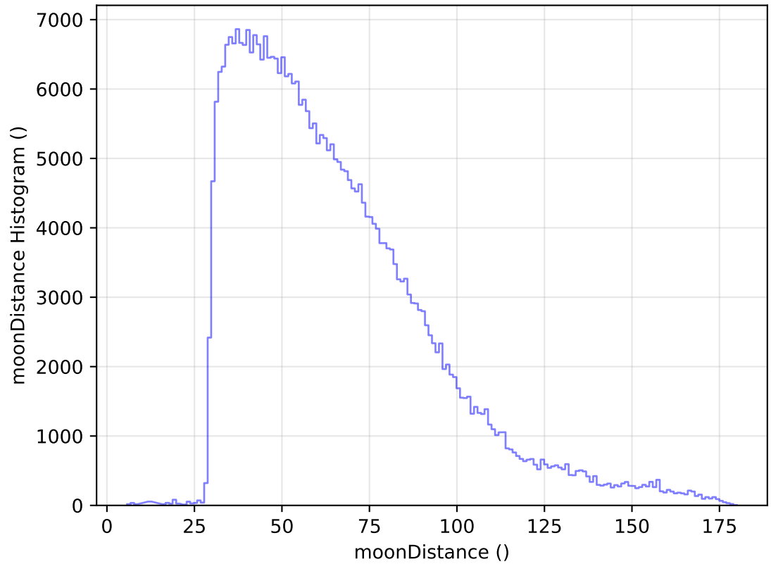
internal_u_expt45_nscale1.1v3.4_10yrs WFD y band: moonDistance Histogram
