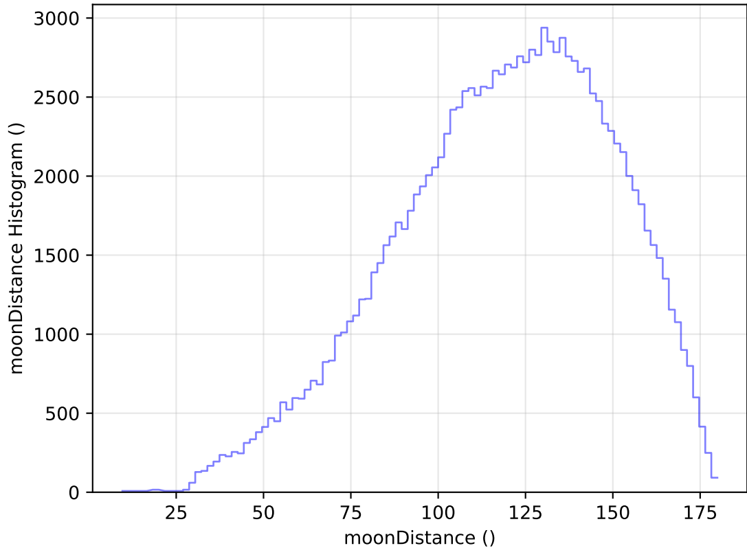
internal_u_expt45_nscale1.1v3.4_10yrs WFD u band: moonDistance Histogram
