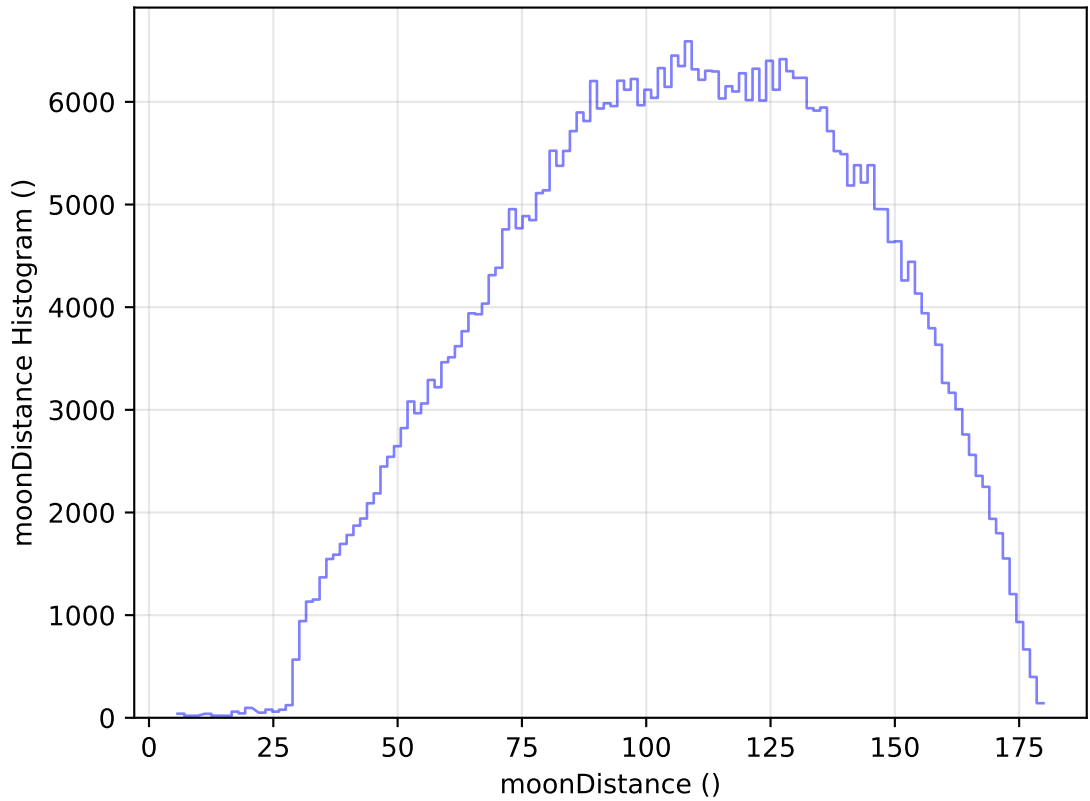
internal_u_expt45_nscale1.1v3.4_10yrs WFD r band: moonDistance Histogram
