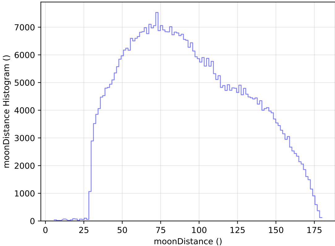
internal_u_expt45_nscale1.1v3.4_10yrs WFD i band: moonDistance Histogram
