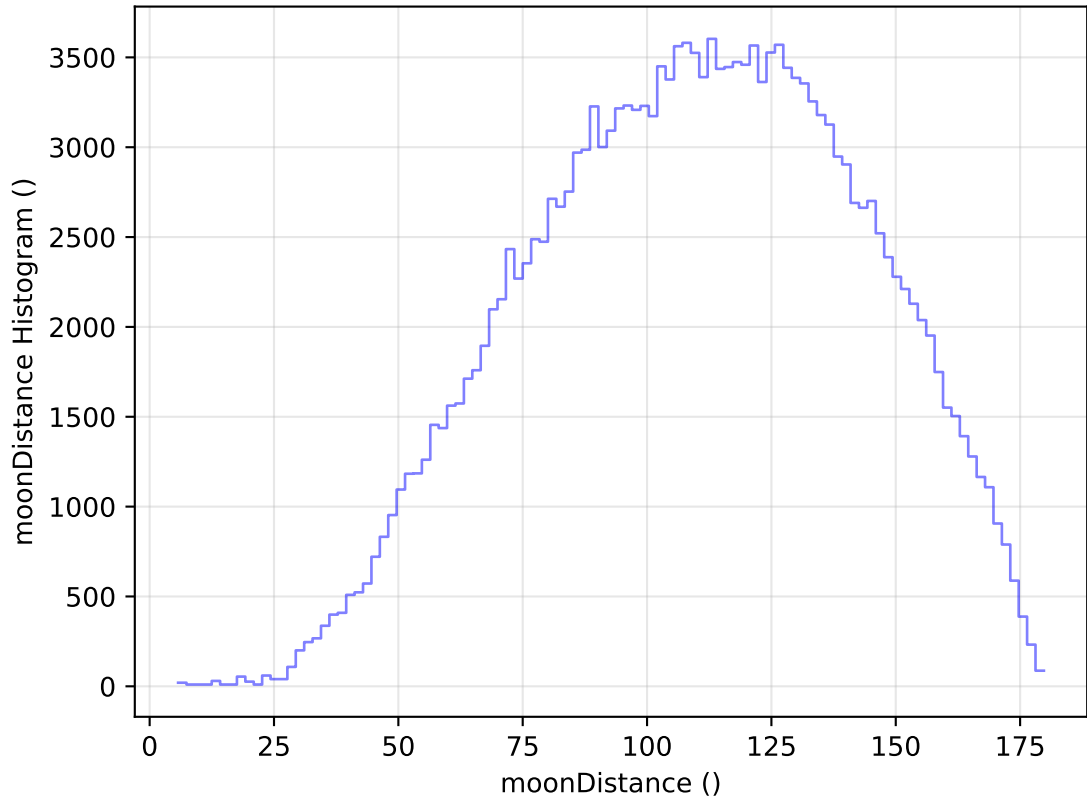
internal_u_expt45_nscale1.1v3.4_10yrs WFD g band: moonDistance Histogram
