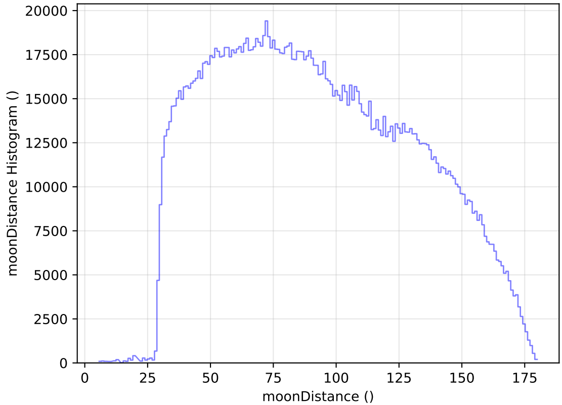
internal_u_expt45_nscale1.1v3.4_10yrs WFD all bands: moonDistance Histogram
