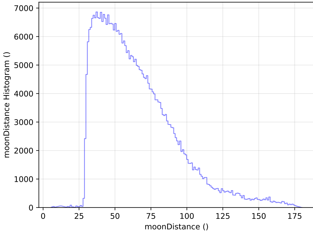
internal_u_expt45_nscale1.1v3.4_10yrs All sky y band: moonDistance Histogram
