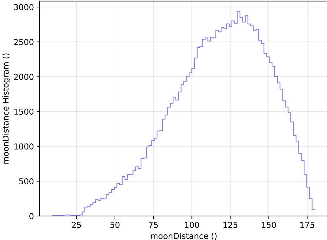
internal_u_expt45_nscale1.1v3.4_10yrs All sky u band: moonDistance Histogram
