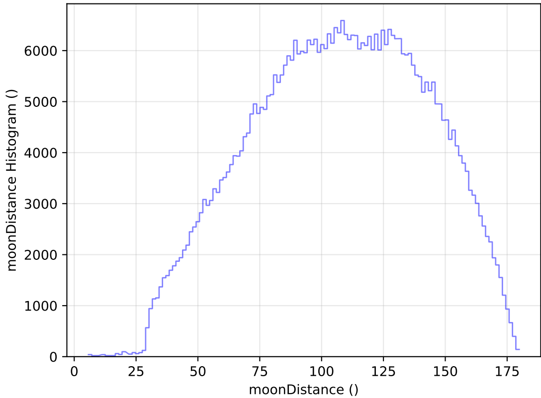
internal_u_expt45_nscale1.1v3.4_10yrs All sky r band: moonDistance Histogram
