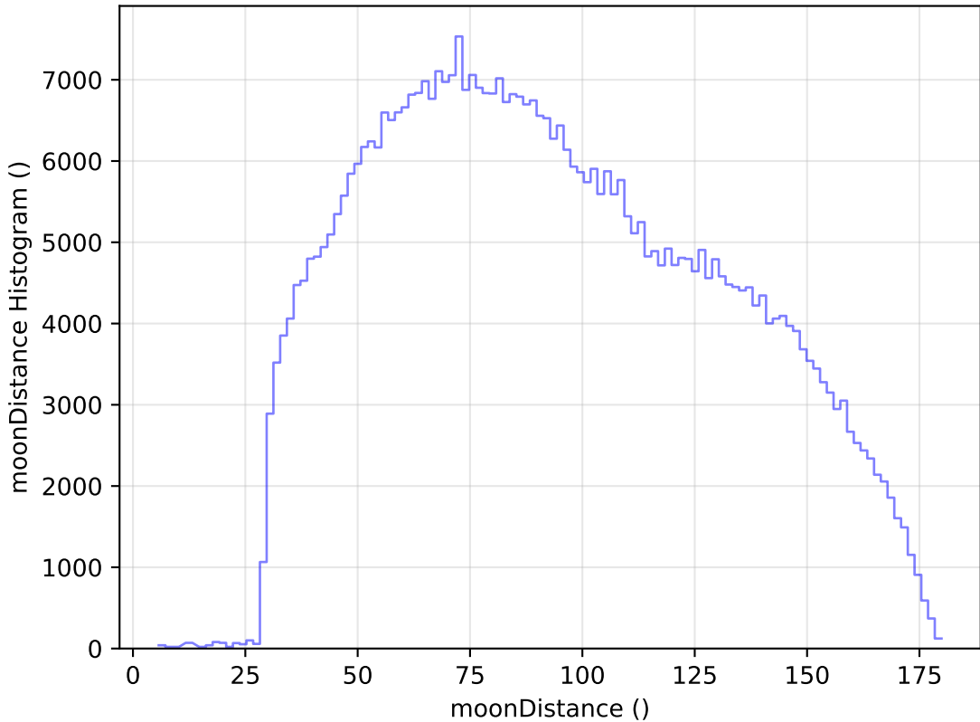
internal_u_expt45_nscale1.1v3.4_10yrs All sky i band: moonDistance Histogram
