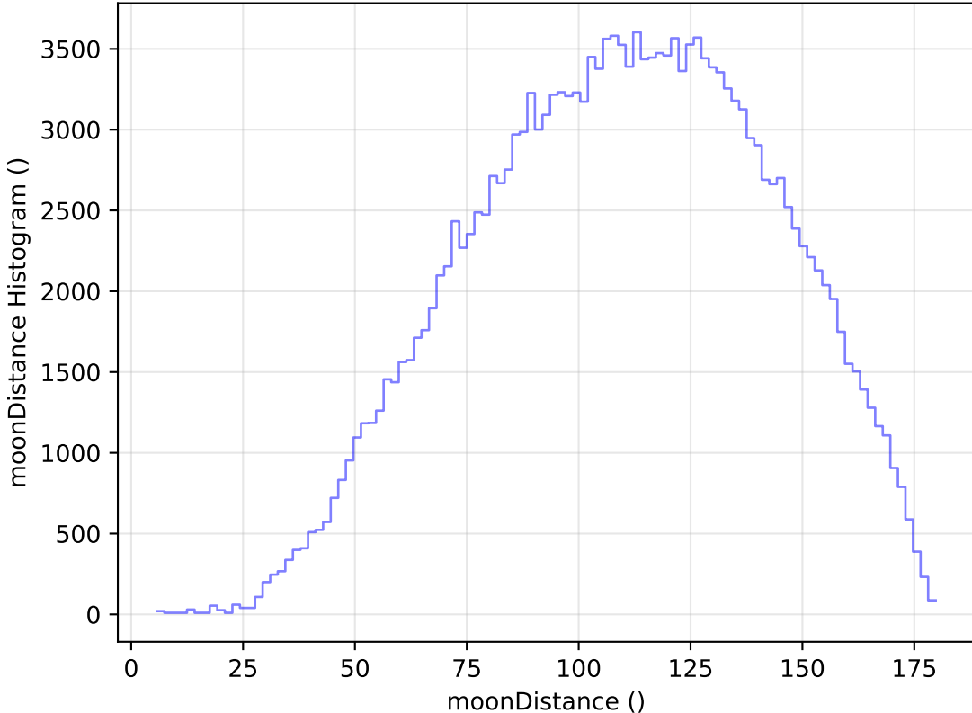
internal_u_expt45_nscale1.1v3.4_10yrs All sky g band: moonDistance Histogram
