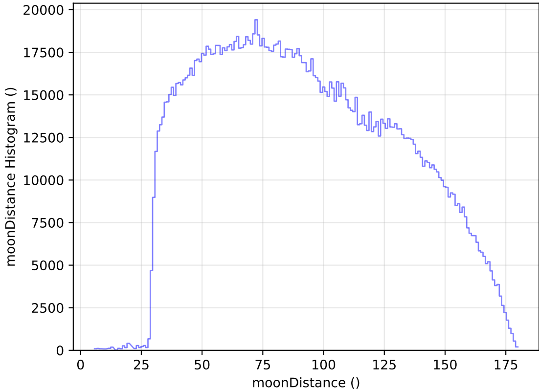
internal_u_expt45_nscale1.1v3.4_10yrs All sky all bands: moonDistance Histogram
