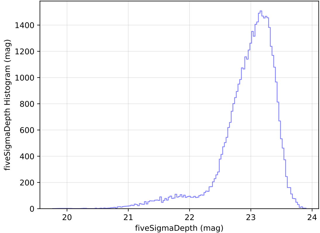
internal_u_expt45_nscale1.1v3.4_10yrs Yr 1 z band: fiveSigmaDepth Histogram
