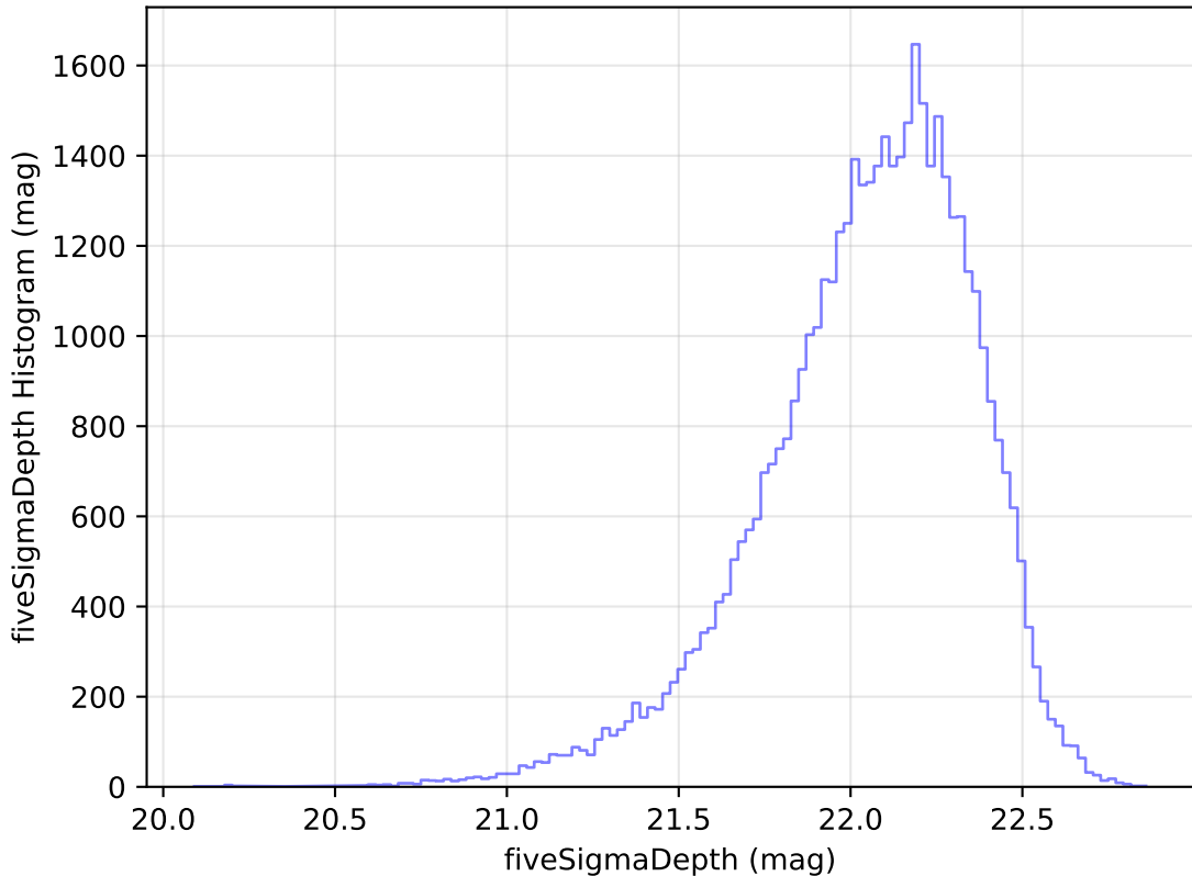
internal_u_expt45_nscale1.1v3.4_10yrs Yr 1 y band: fiveSigmaDepth Histogram
