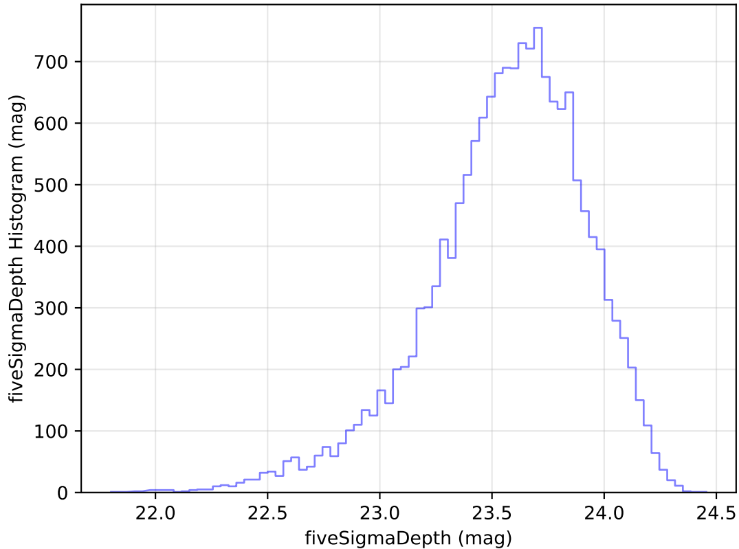
internal_u_expt45_nscale1.1v3.4_10yrs Yr 1 u band: fiveSigmaDepth Histogram
