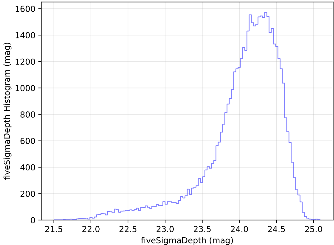
internal_u_expt45_nscale1.1v3.4_10yrs Yr 1 r band: fiveSigmaDepth Histogram
